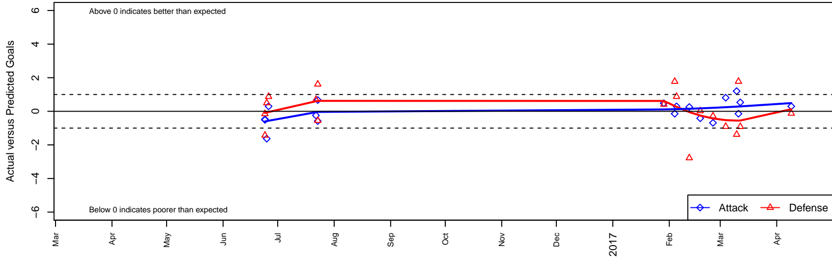
THUSC United Mercury G02 Dots are actual minus expected GF (blue circles) and GA (red triangles). Blue line is smoothed change in attack strength. Red is smoothed change in defense strength.
